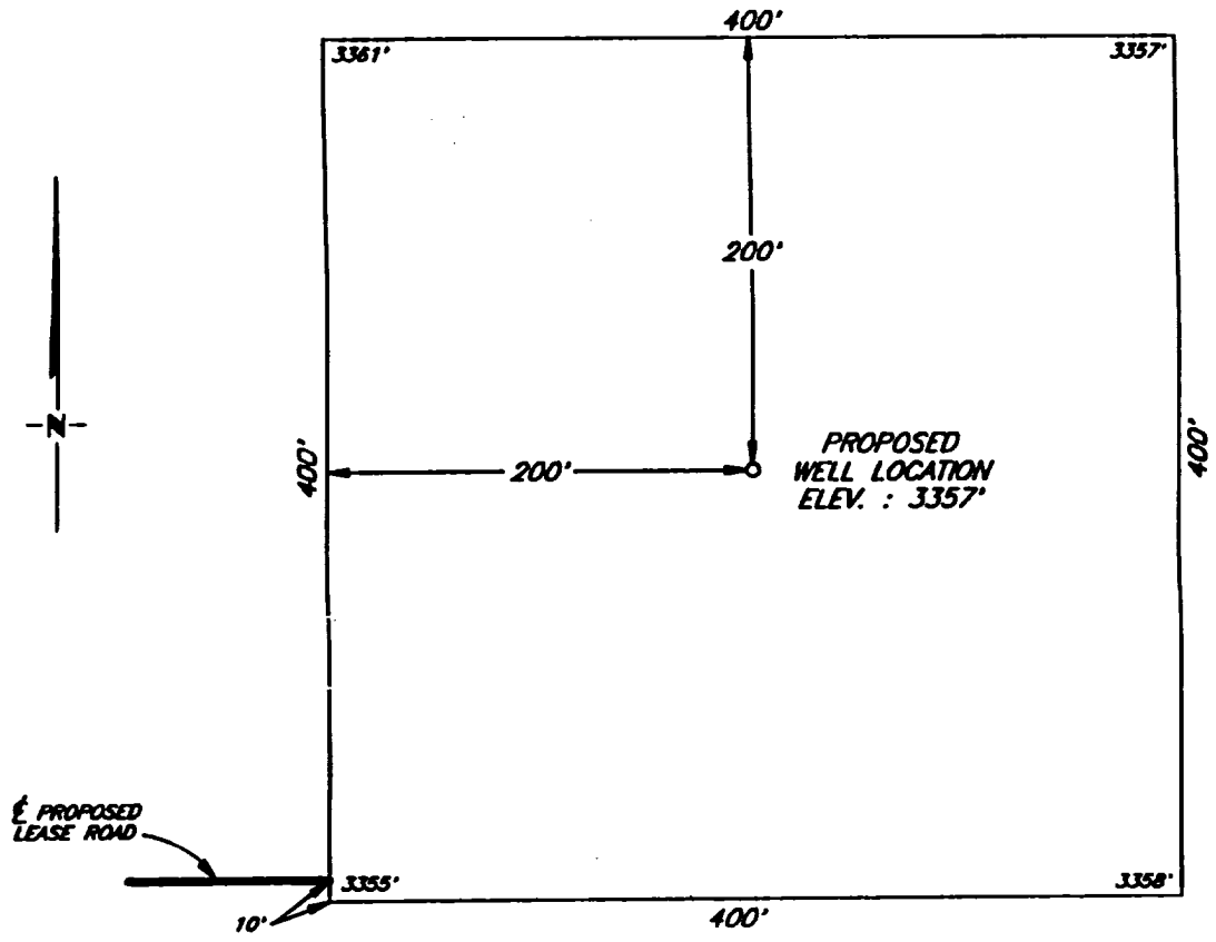
DETAIL VIEW 1" = 100'
