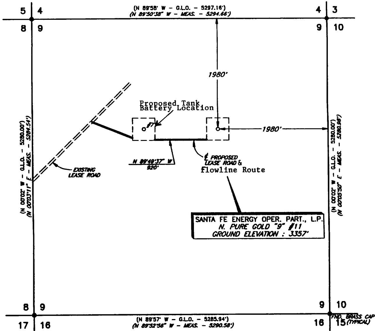
PLAN VIEW 1" = 1000'
