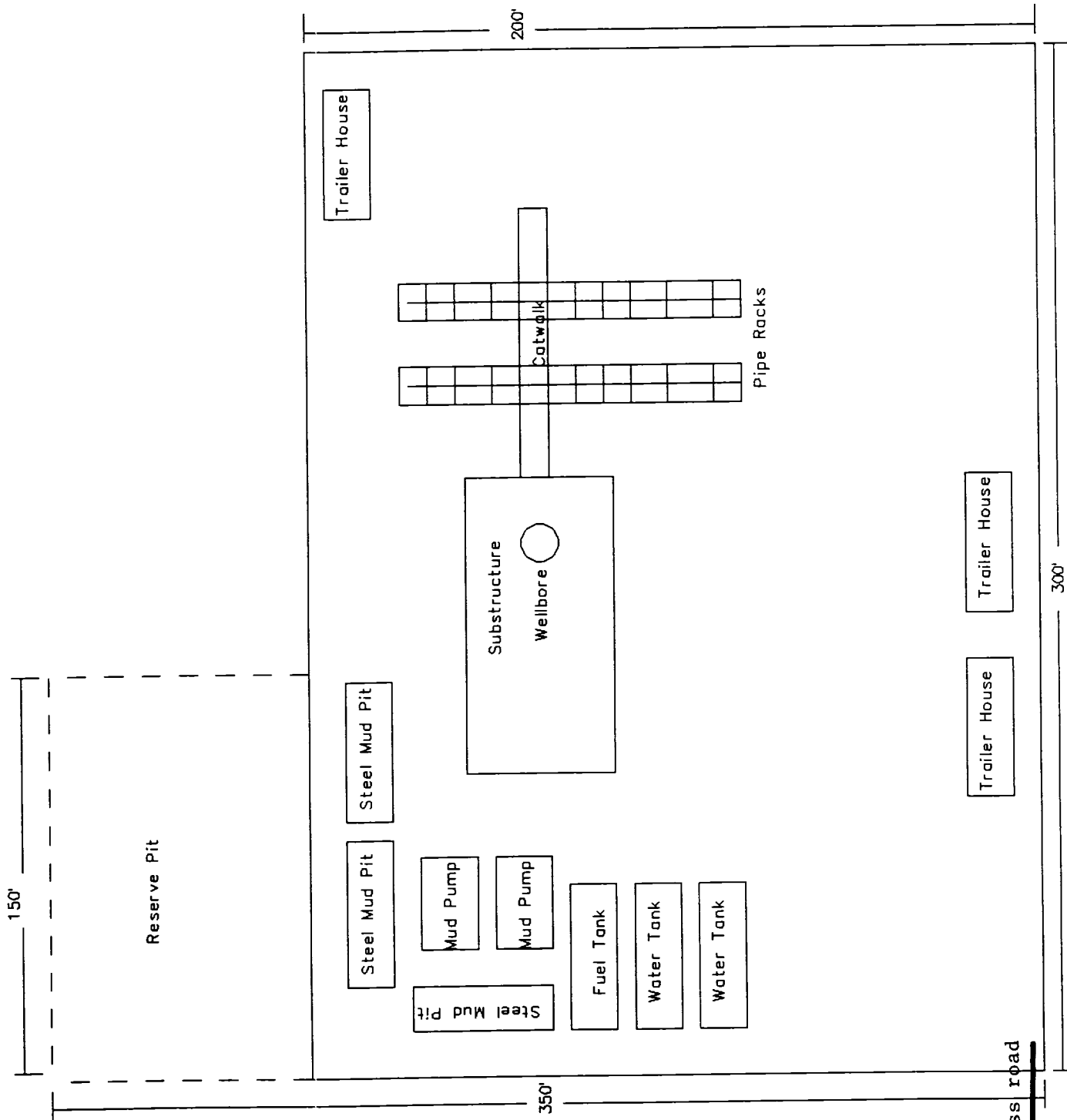
EXHIBIT H WELL SITE LAYOUT SANTA FE ENERGY OPERATING PARTNERS, L.P. N. PURE GOLD "9" FED NO. 13 SEC 9, T-23-S,R-31-E EDDY COUNTY, NEW MEXICO
