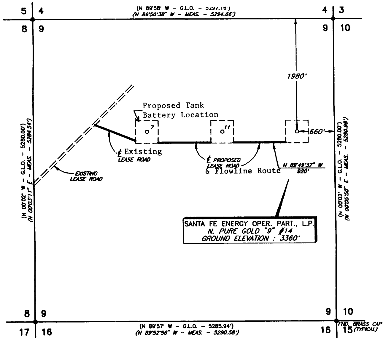
PLAN VIEW 1" = 1000'
