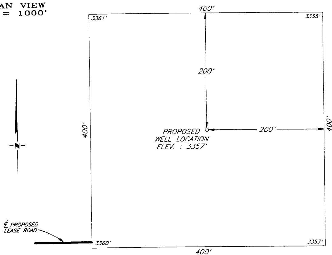
DETAIL VIEW 1" = 100'
