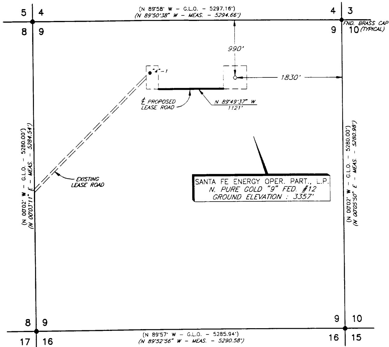
PLAN VIEW 1" = 1000'
