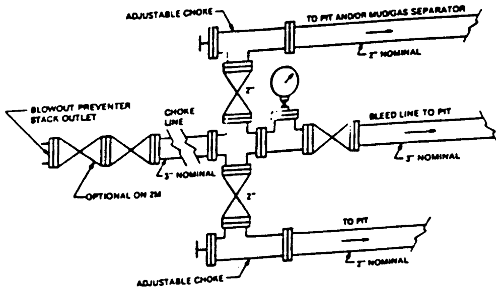
FIGURE K4-1. Typical choke manifold assembly for 2M and 3M ram working pressure service — surface installation.
