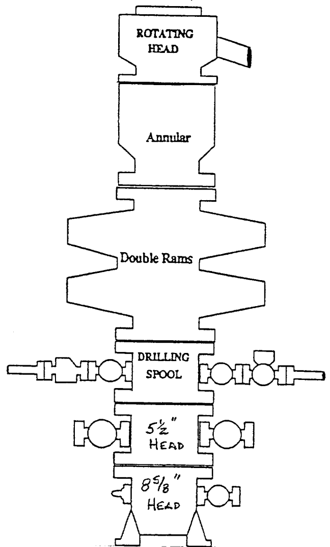
4 3/4" HORIZONTAL HOLE
