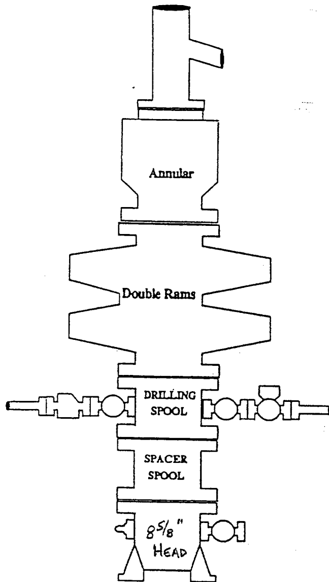
7 7/8" VERTICAL HOLE
