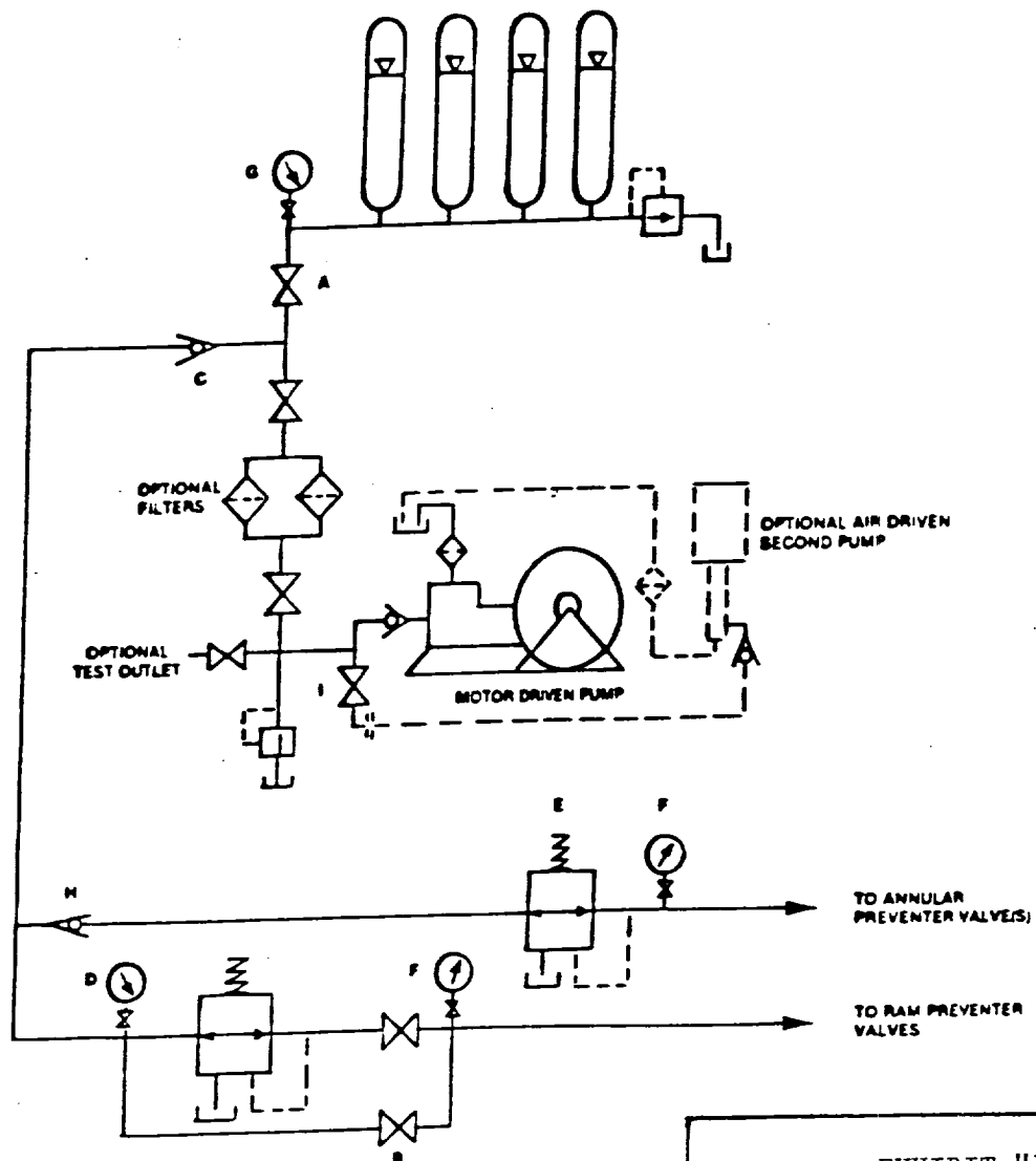
EXHIBIT "1-E" CHOKE MANIFOLD & CLOSING UNIT
