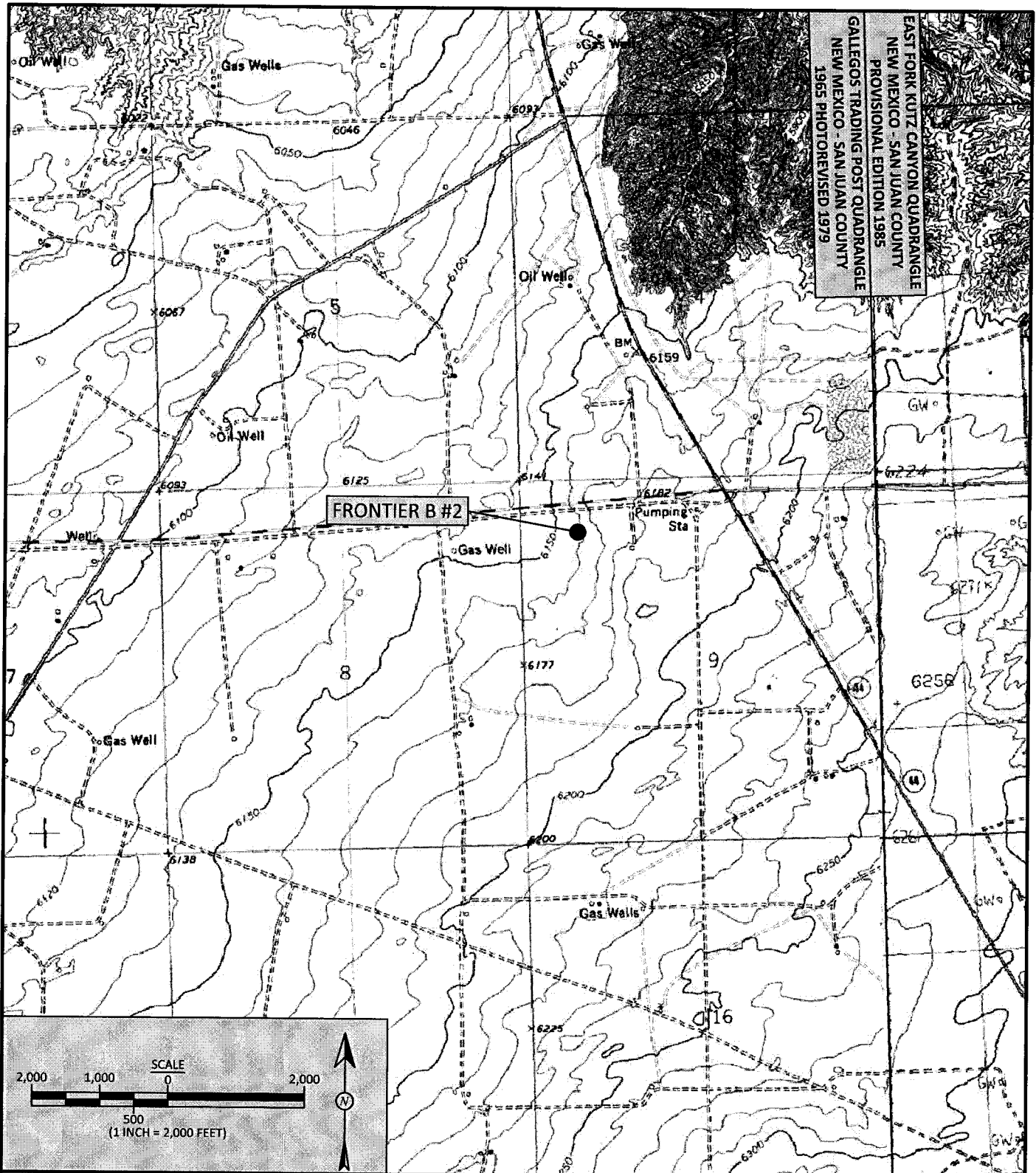
FIGURE 1 TOPOGRAPHIC SITE LOCATION MAP ConocoPhillips FRONTIER B#2 SAN JUAN COUNTY, NEW MEXICO NW¼, NW¼, SECTION 9, T27N, R11W N36.59474°, W108.01488°
