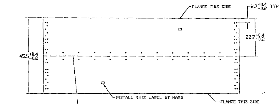
SLIT ON CENTER OF CORR AFTER CORR/PUNCHING MANUFACTURING VIEW ONLY - DOUBLE PANEL AFTER CORR & PUNCH, BEFORE SLITTING & FLANGING
