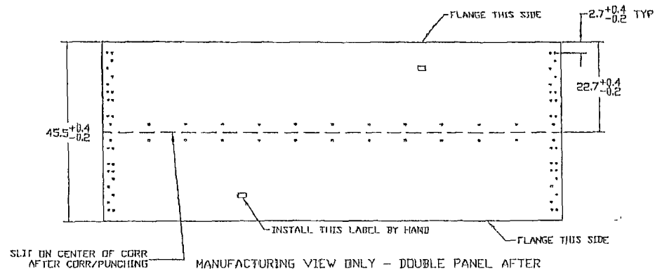
MANUFACTURING VIEW ONLY - DOUBLE PANEL AFTER CORR & PUNCH, BEFORE SLITTING & FLANGING
