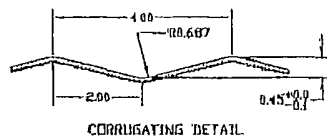
CORRUGATING DETAIL
