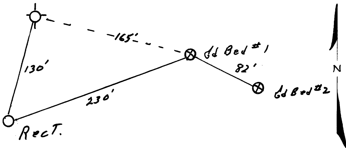
GROUND BED LAYOUT SKETCH
