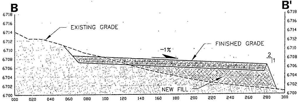
SECTION B-B'
