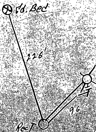
GROUND BED LAYOUT SKETCH
