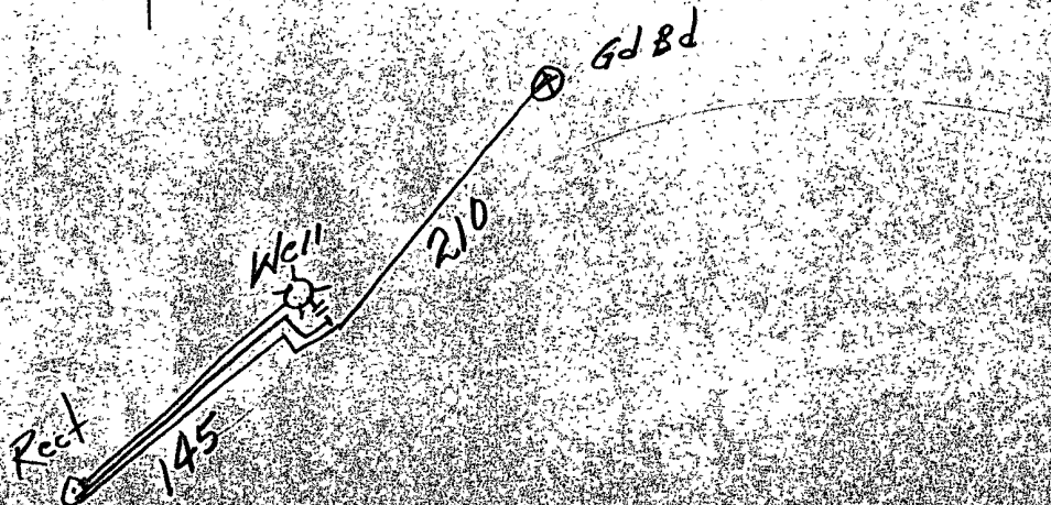
GROUND BED LAYOUT SKETCH
