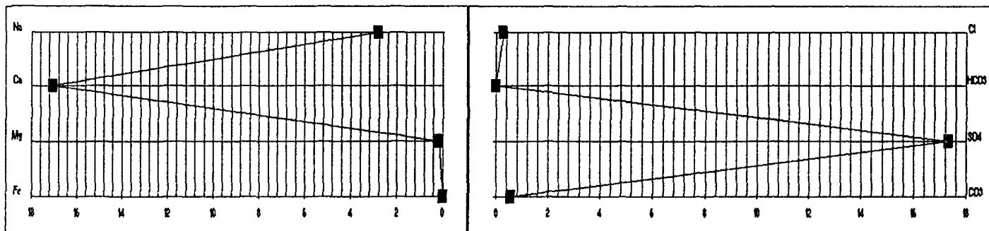
Stiff Diagram
