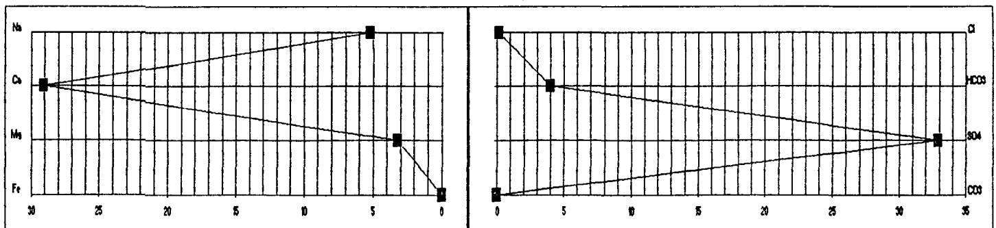
Stiff Diagram
