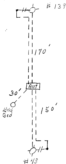
GROUND BED LAYOUT SKETCH
