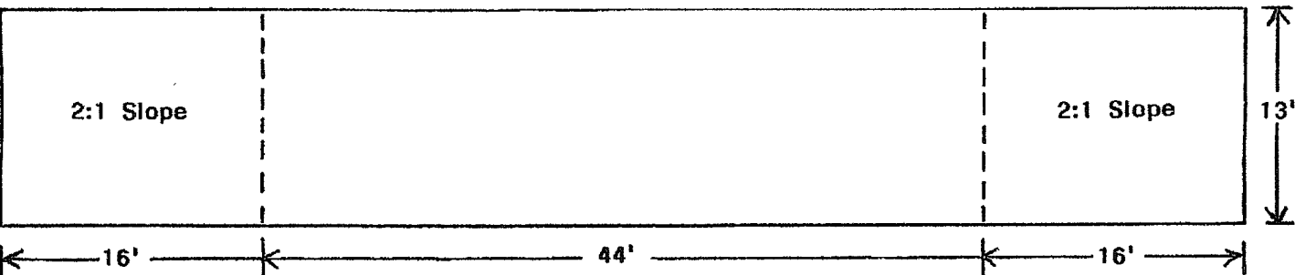
PLAN VIEW
