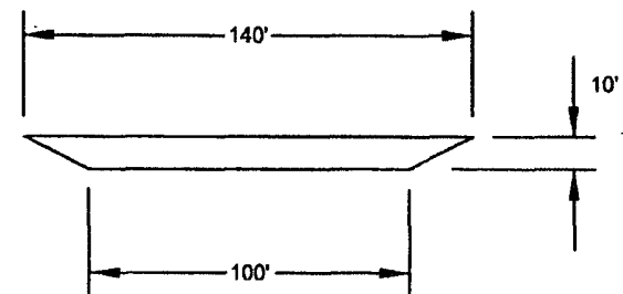
VIEW B-B
