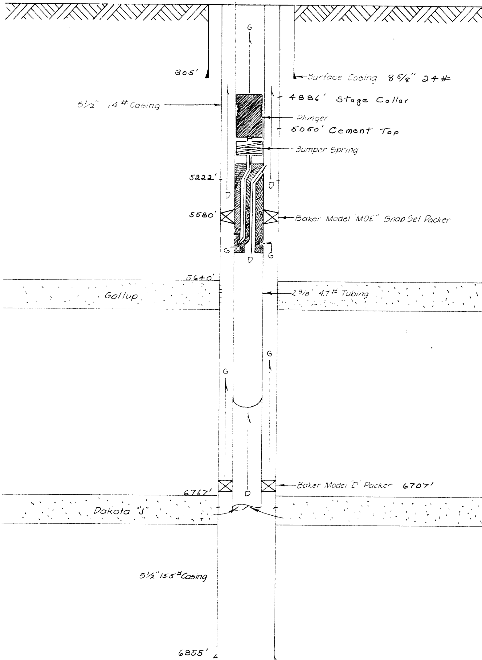
SCHEMATIC DIAGRAM of DUAL COMPLETION of NE HAYNES No. 5 CONTINENTAL OIL CO. Dakota & Gallup Formations.
