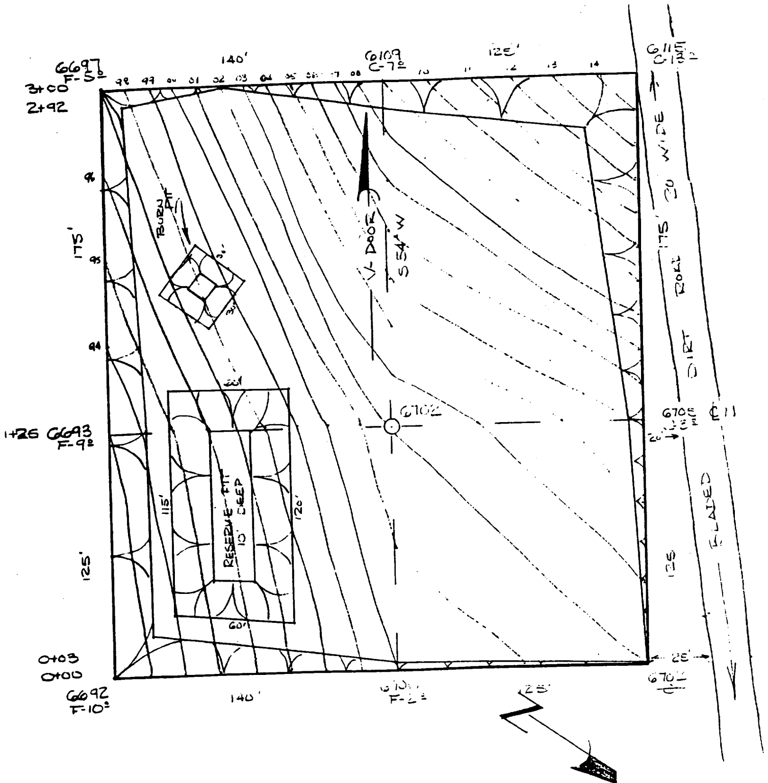
PAD LAYOUT AND TOPOGRAPHY
