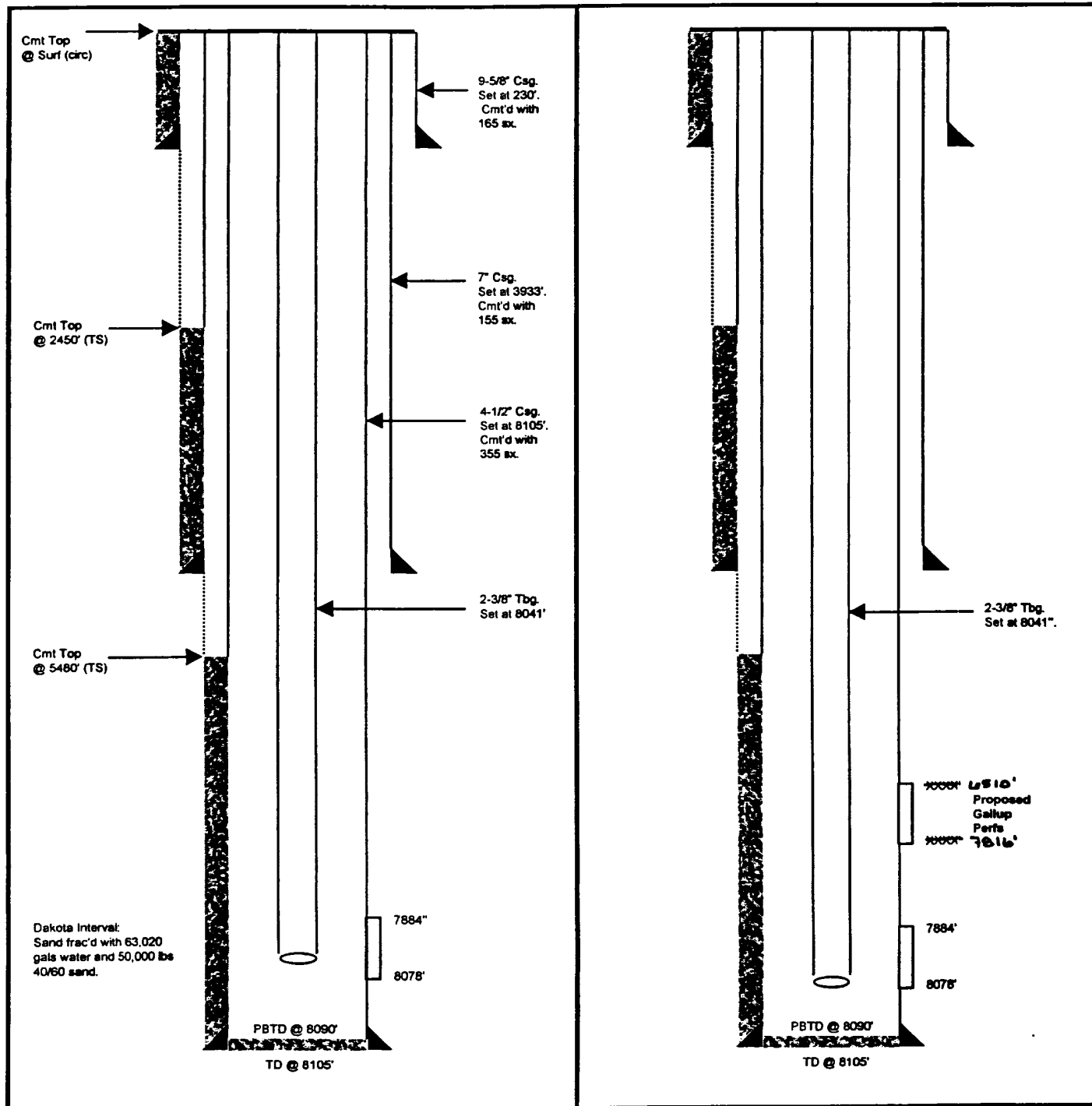
Proposed Schematic
