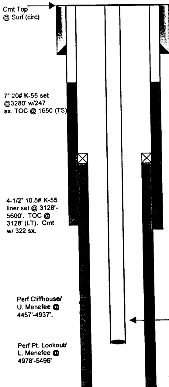
Current Schematic
