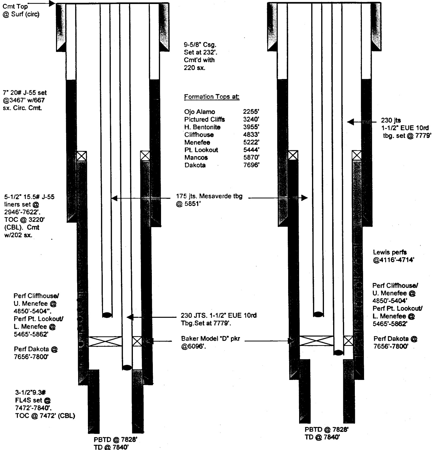
Current Schematic
