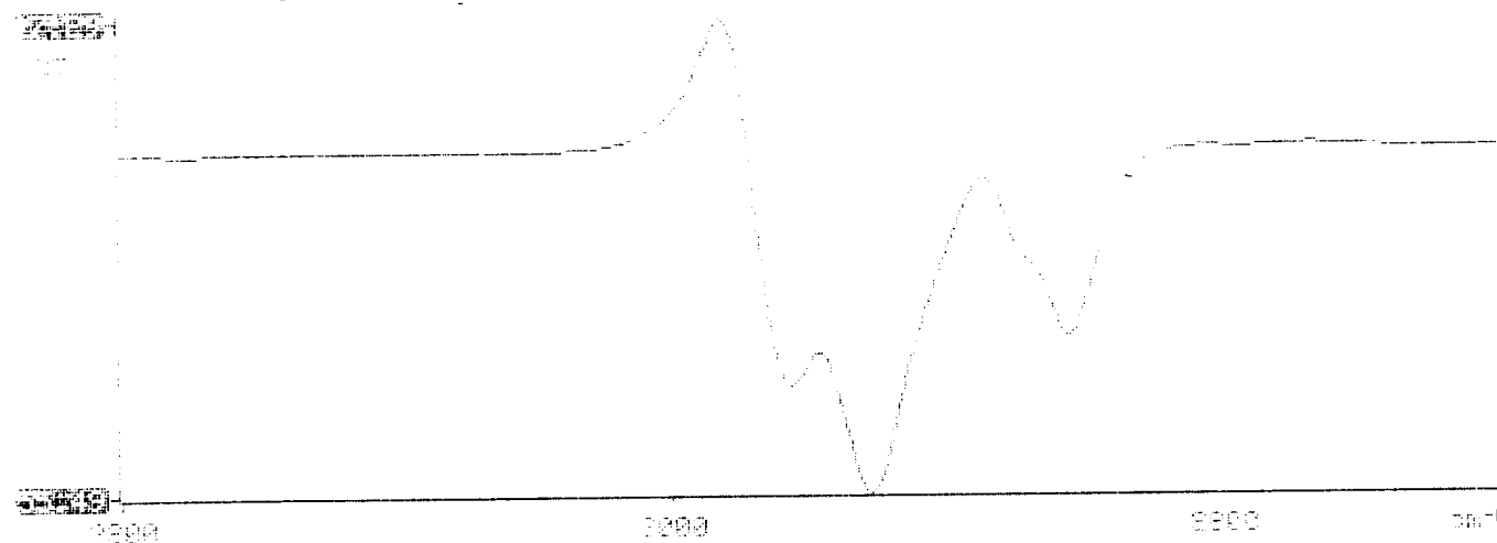
Oil Petroleum Hydrocarbons spectrum
