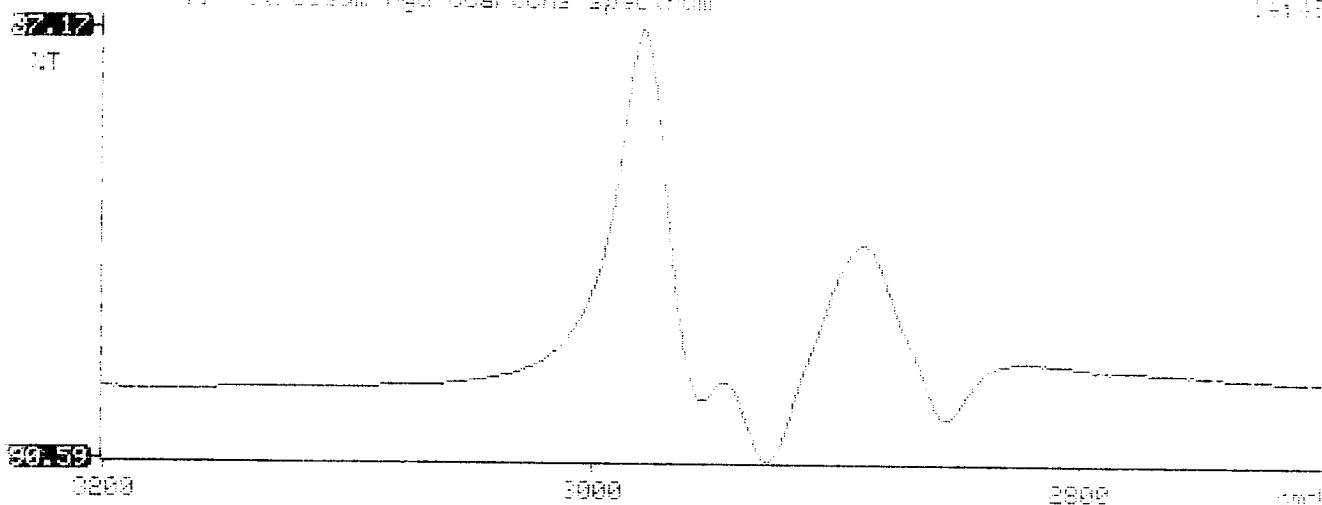
W: Petroleum hydrocarbons spectrum
