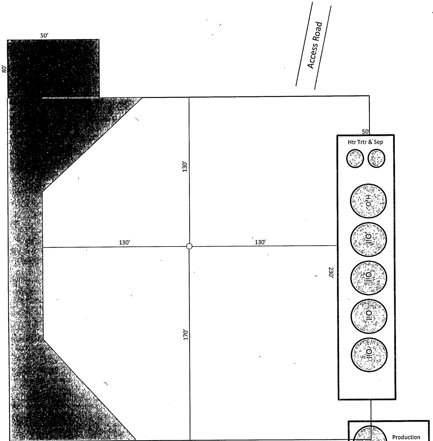
Exhibit D-1 Production Facilities Layout Diagram North Maduro Federal Unit No. 5 Cimarex Energy Co. of Colorado 20-19S-33E SHL 660 FSL & 330 FEL BHL 660 FSL & 330 FWL Lea County, NM
