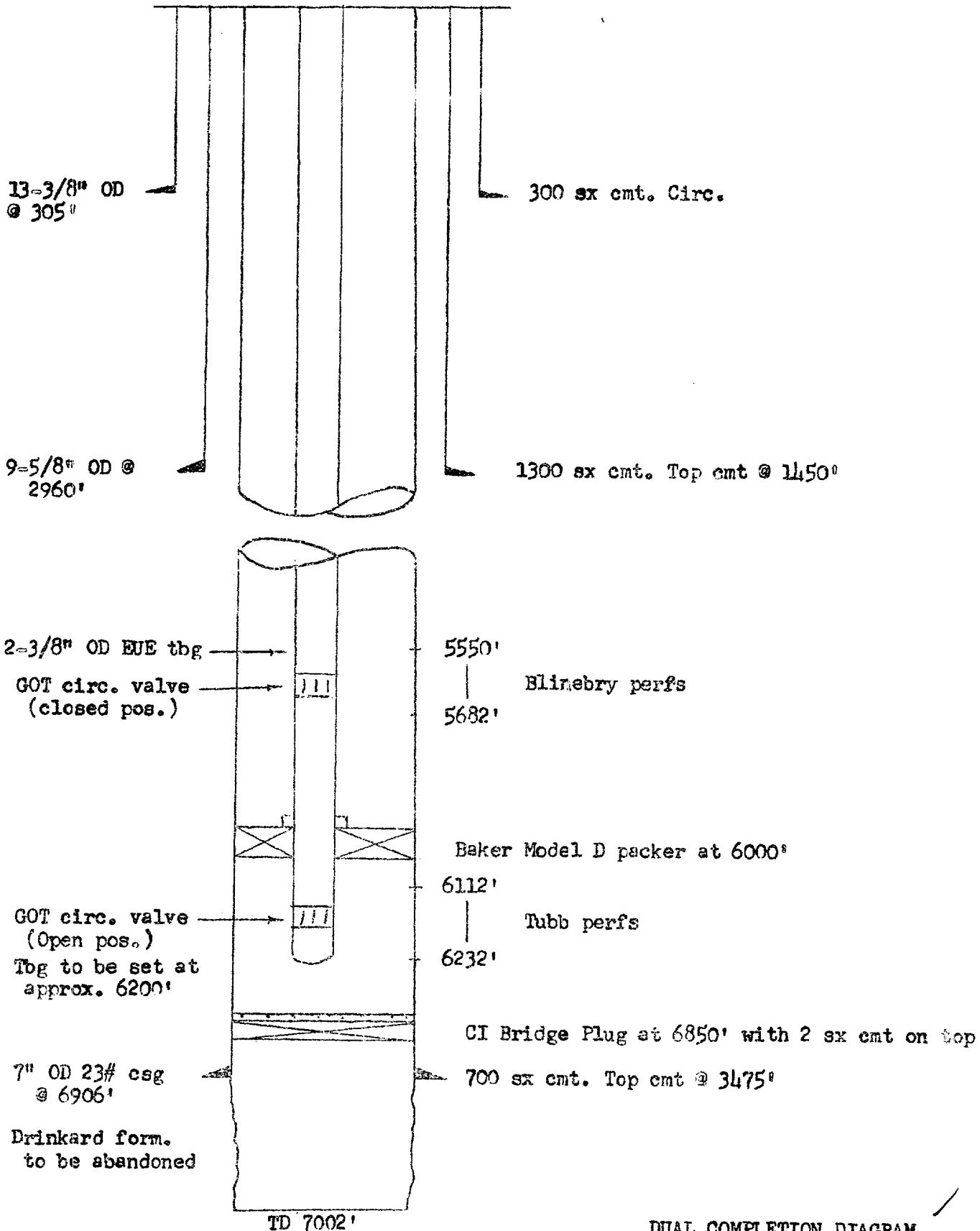
DUAL COMPLETION DIAGRAM GULF OIL CORPORATION - EVELYN LINEBERRY NO. 1 BLINEBRY GAS - TUBB GAS
