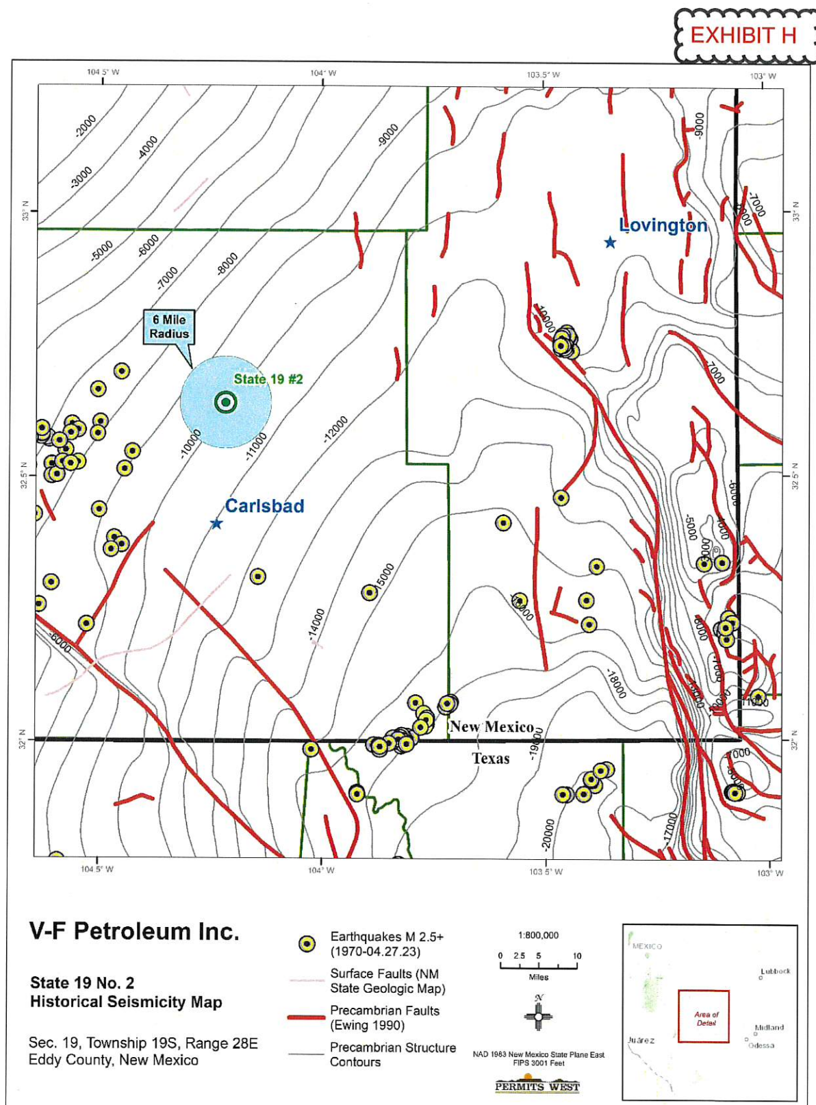
Figure 1. Structural contour map of the Precambrian basement in feet below sea level. Red lines represent the locations of Precambrian basement-penetrating faults (Ewing et al., 1990). The State 19 SWD #2 well lies ~18 miles NE of the closest deeply penetrating fault and 14 miles from the closest historic earthquake.
