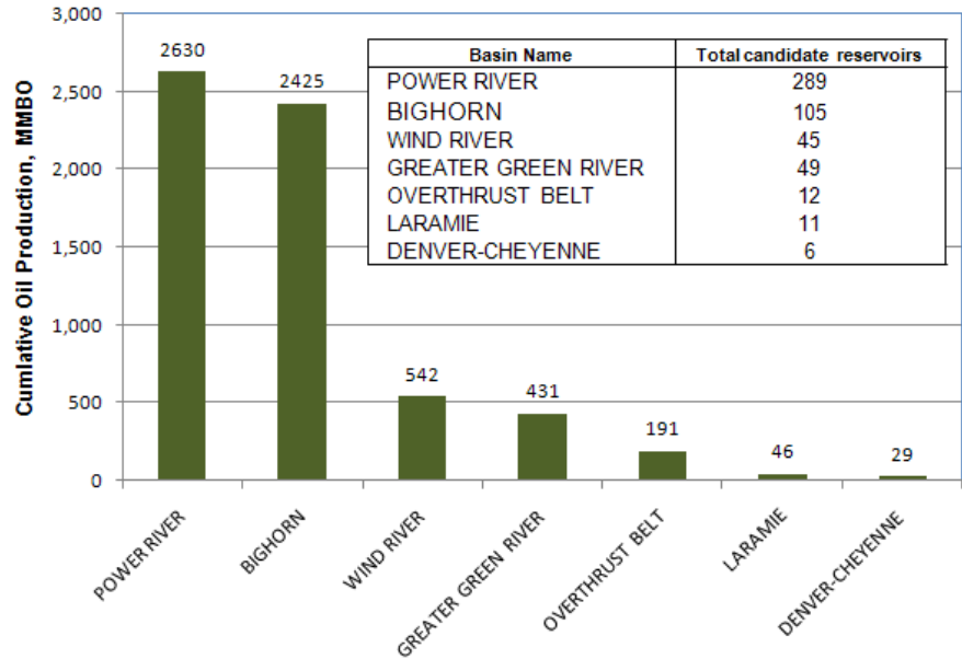
Figure 2. Number of CO 2 -EOR candidate reservoirs and their cumulative oil productions by Wyoming basins
