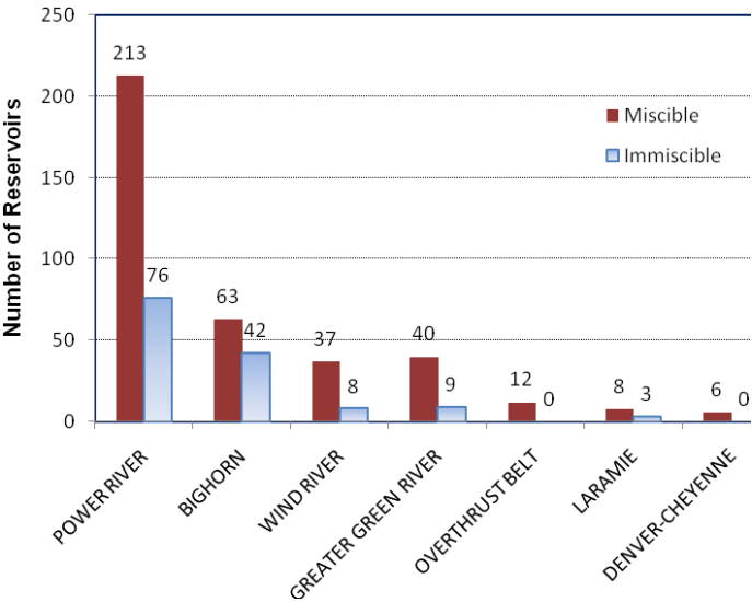
Figure 3. Number of miscible and immiscible CO 2 -EOR candidate reservoirs by Wyoming basins
