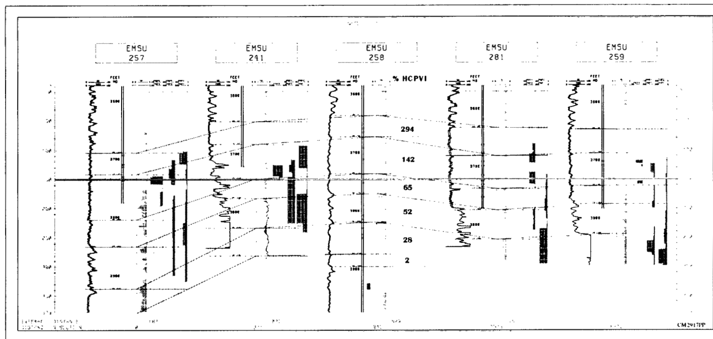
Fig. 3. — Structural cross-section.
