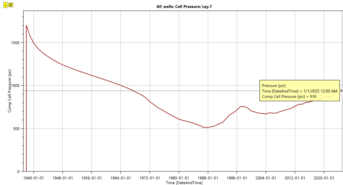
Grayburg historical pressure history
