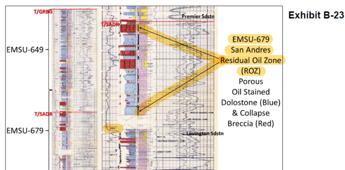
Left Figure: Combined EMSU-649 and EMSU-679 well logs and core descriptions that contain the complete Grayburg reservoir and upper San Andres residual oil zone (ROZ) to beneath the Lovington Sandstone. Right Figure: Close-up of EMSU-679 well log and core from Premier Sandstone at the base of Grayburg reservoir down section, crossing basal lag conglomerate (top red) and unconformity (red line) that separates Grayburg reservoir from upper San Andres residual oil zone (ROZ). Top of San Andres is at 4144 ft (-548 ft). Base of cored interval is 4358 ft (-762 ft). Black arrows point to top and bottom of porous, oil-stained residual oil zone (ROZ) in San Andres ROZ.
