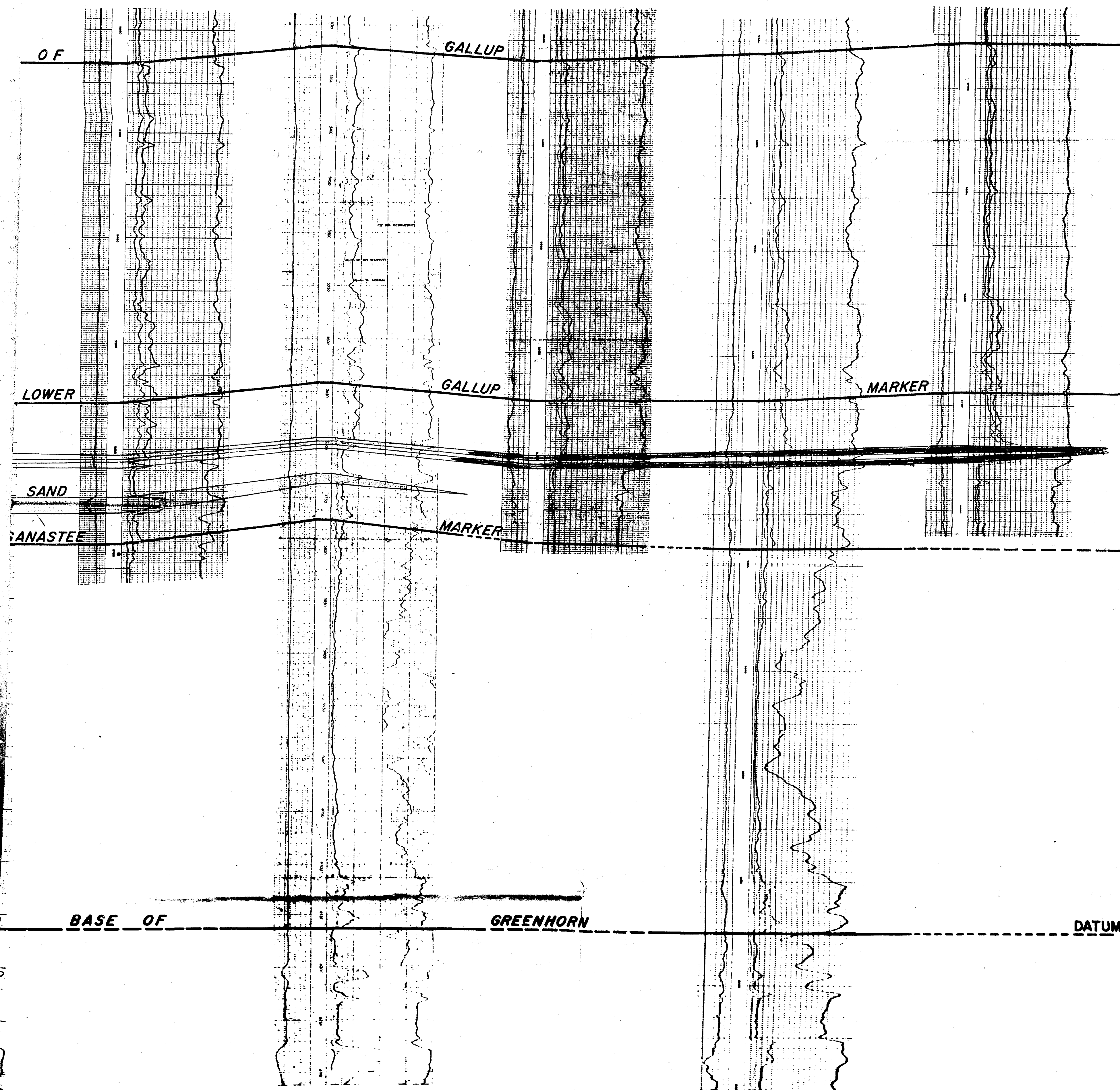
STRTAGRAPHIC CROSS-SECTION THROUGH PIÑON GALLUP OIL POOL SAN JUAN COUNTY, NEW MEXICO
