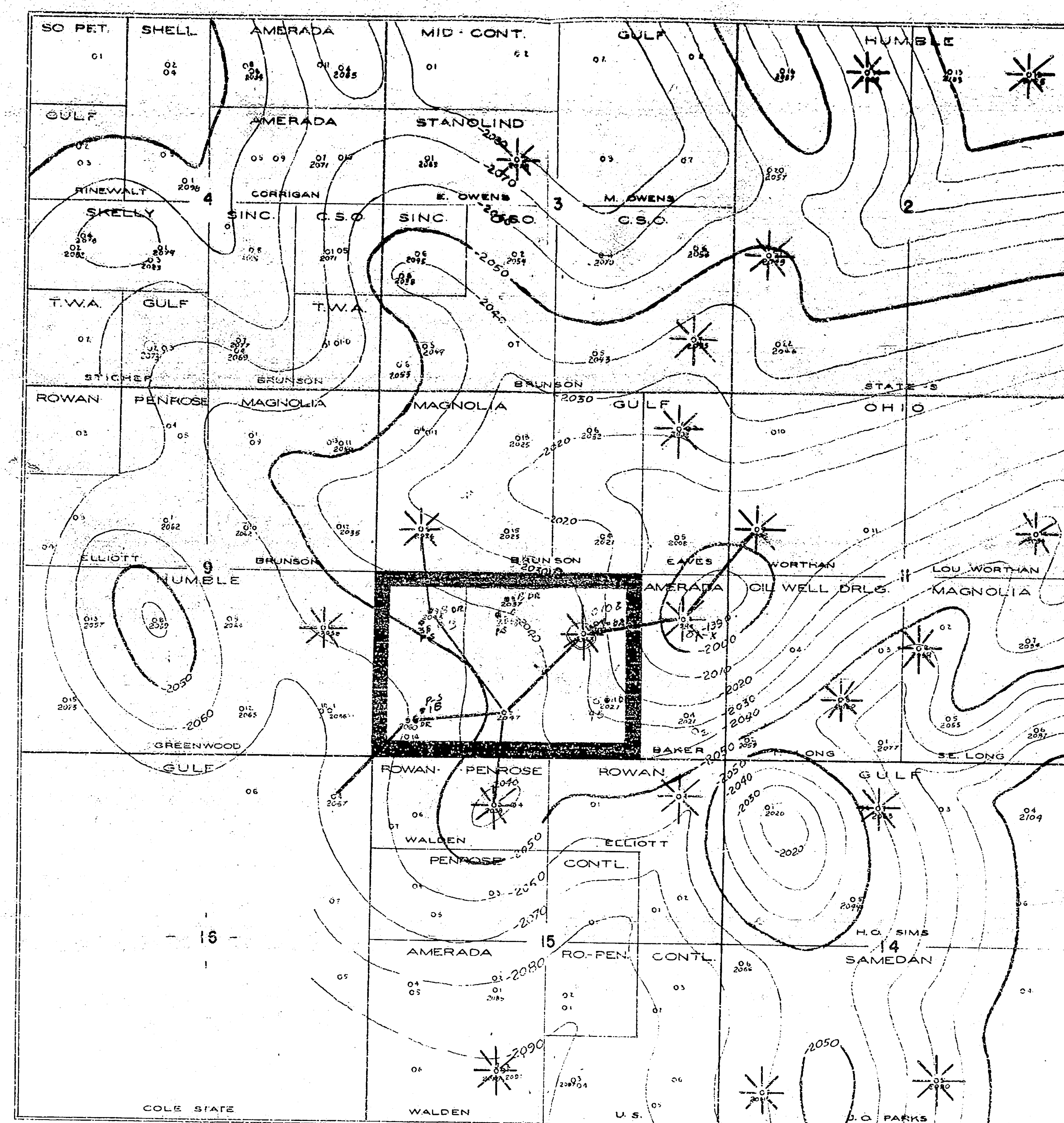
BLINEBRY STRUCTURE MAP 10' CONTOUR INTERVAL
