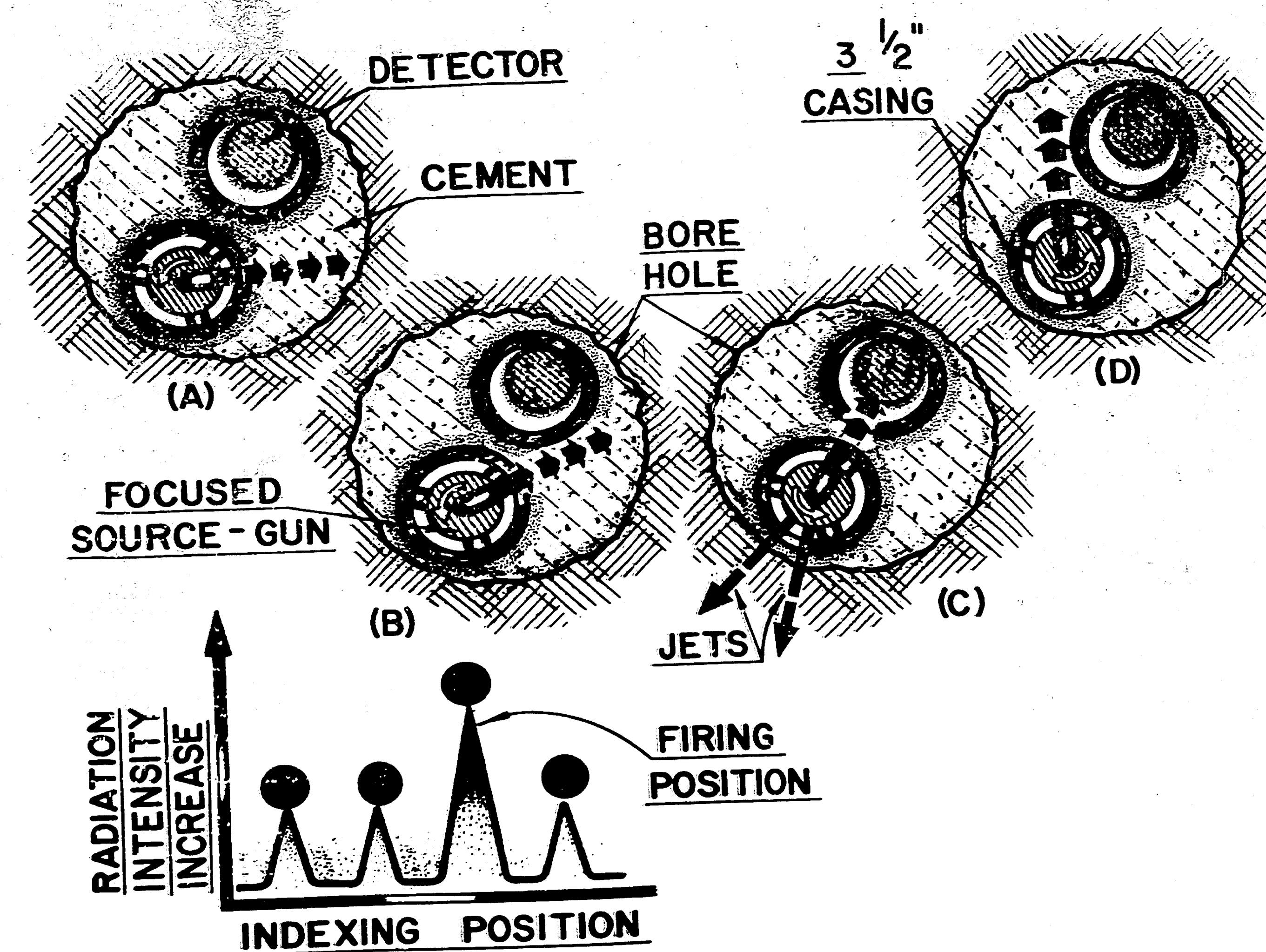
Principle Of Operation Of Self-Orienting Radiation Device
