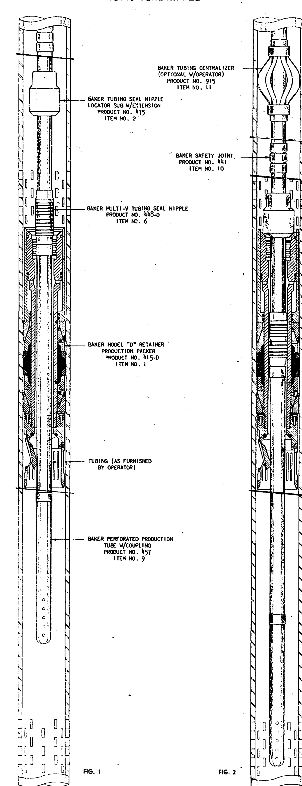
TWO ZONE PRODUCTION METHOD USING A BAKER MODEL "D" RETAINER PRODUCTION PACKER, A TUBING SEAL NIPPLE LOCATOR SUB WITH EXTENSION AND ONE MULTI-V TUBING SEAL NIPPLE.
