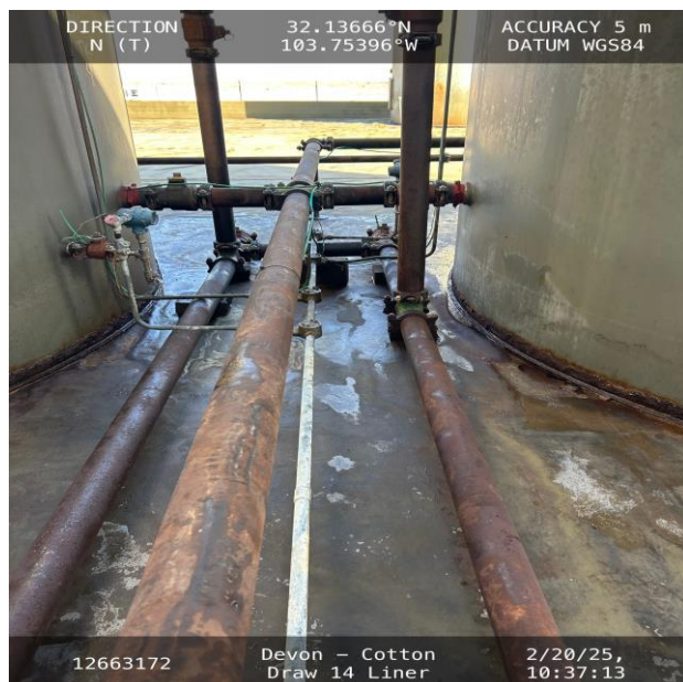
Photo 13 View of interior containment facing north.
