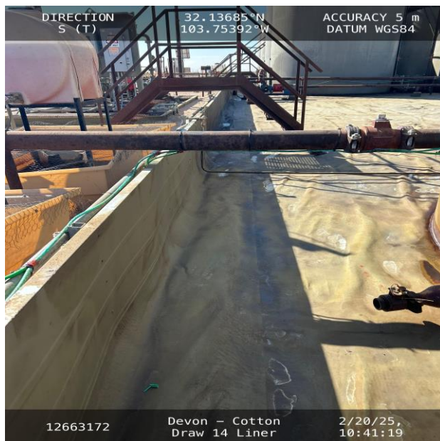
Photo 19 View of eastern side of secondary containment facing south.
