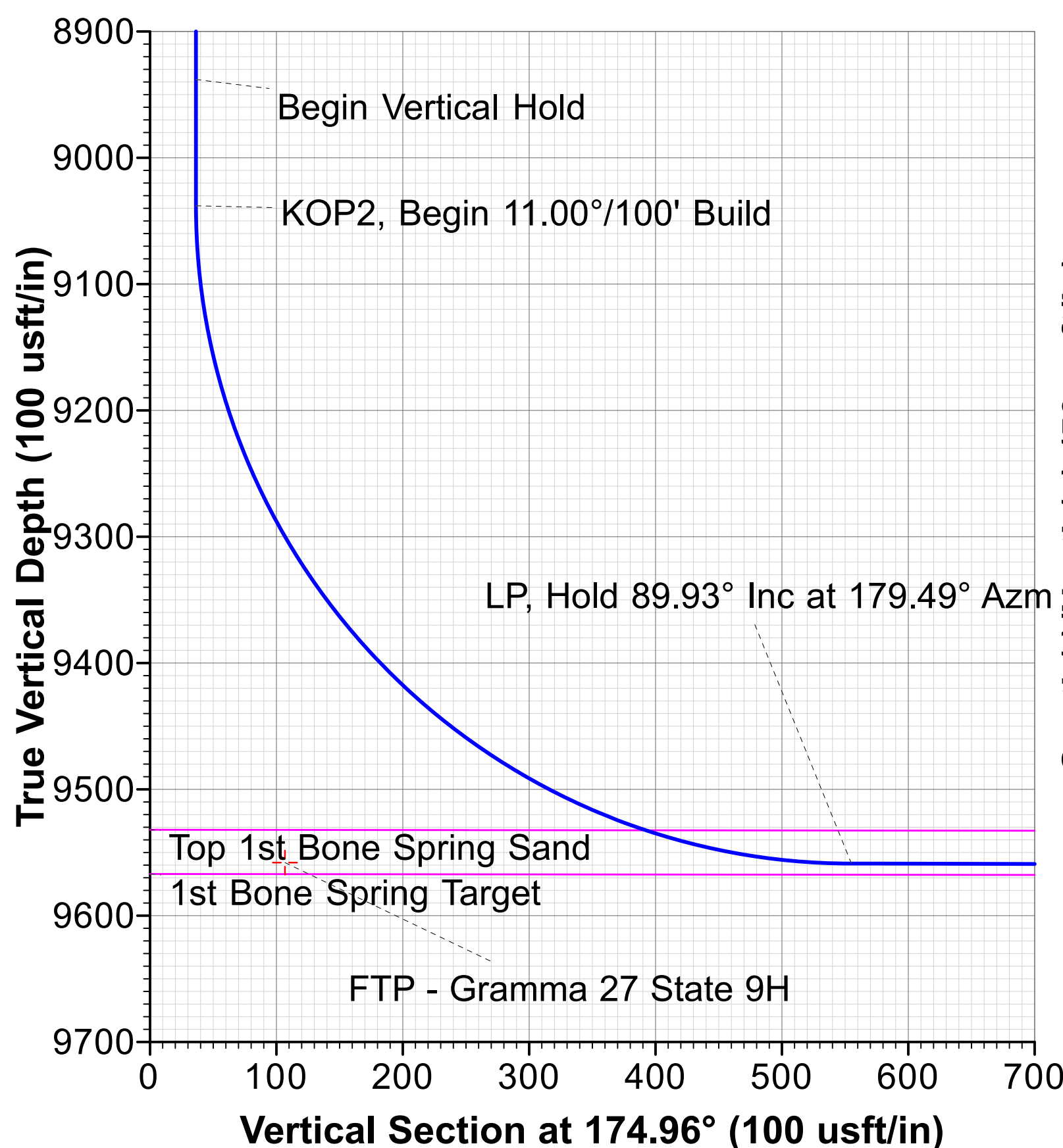
Vertical Section at 174.96° (100 usft/in)
