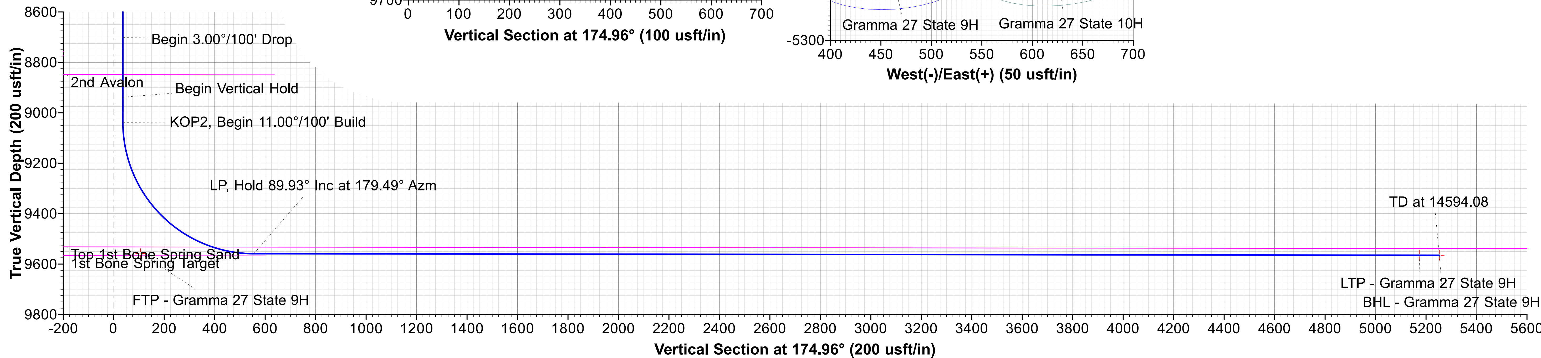
Vertical Section at 174.96° (200 usft/in)
