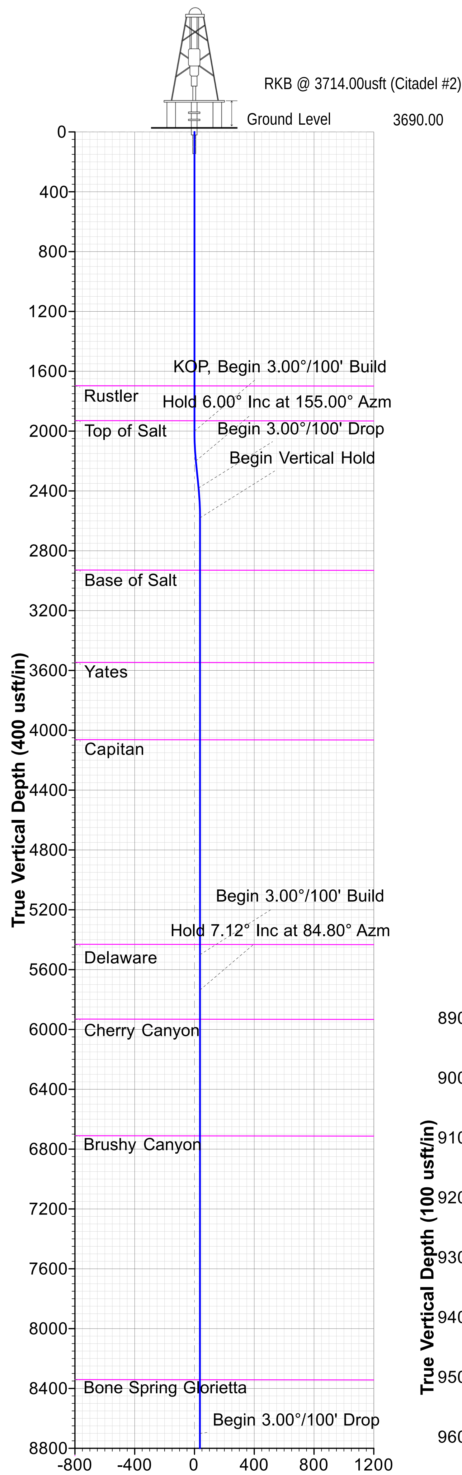
Vertical Section at 174.96° (400 usft/in)
