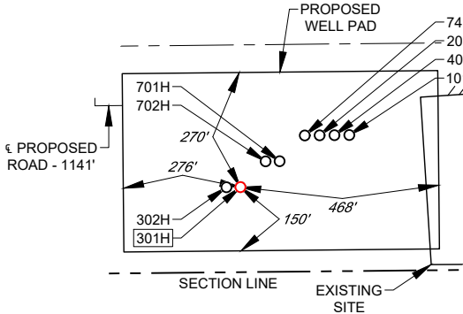
DETAIL VIEW SCALE: 1" = 400'
