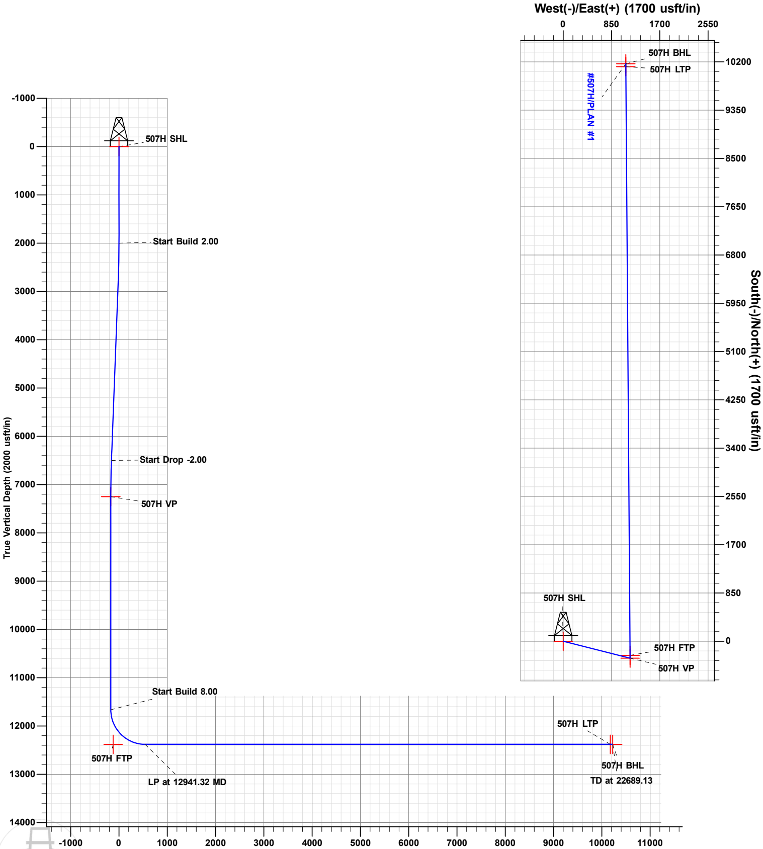
Vertical Section at 6.19° (2000 usft/in)
