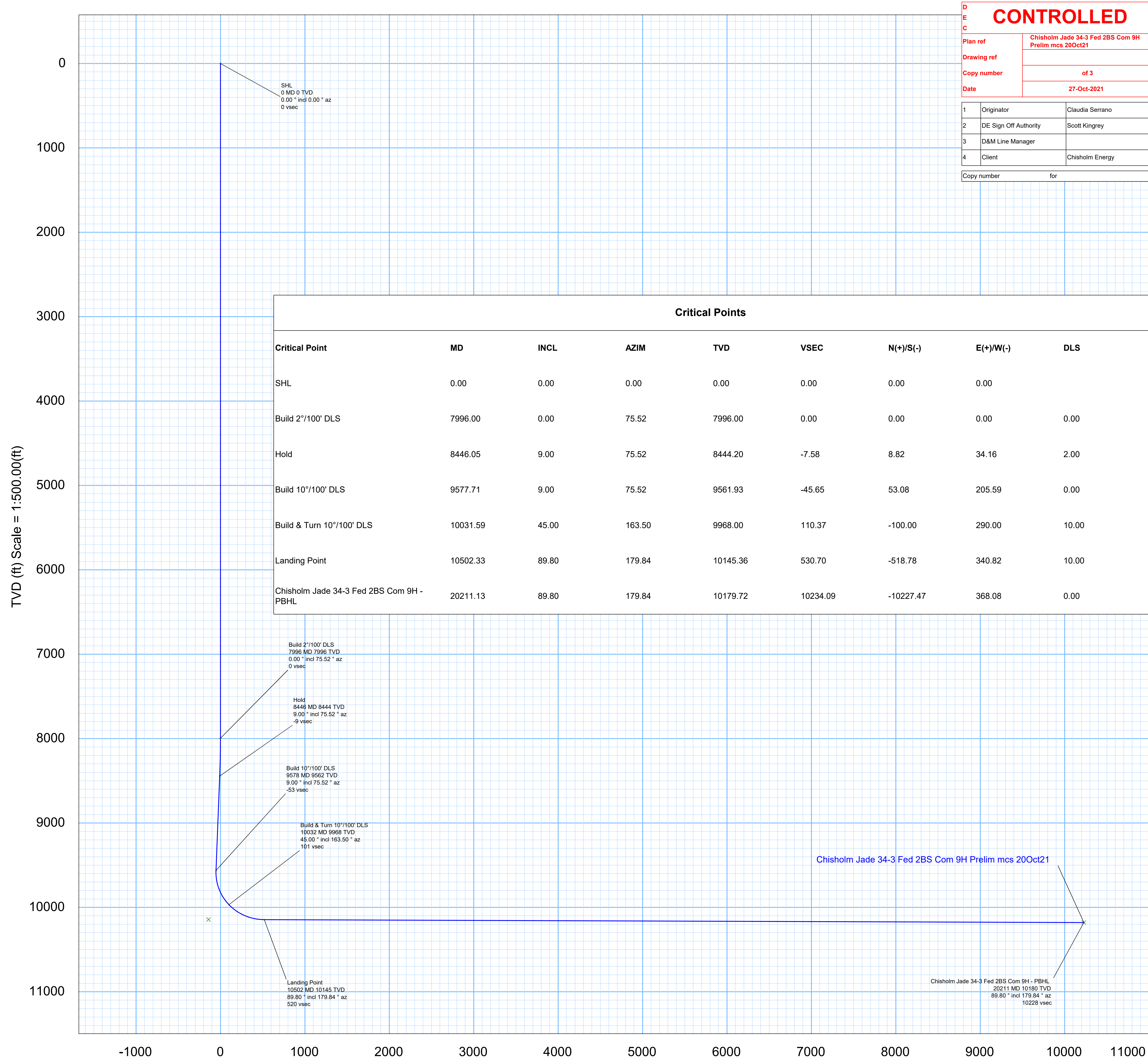
Vertical Section (ft) Azim = 179.84° Scale = 1:500.00(ft) Origin = 0N/-S, 0E/-W
