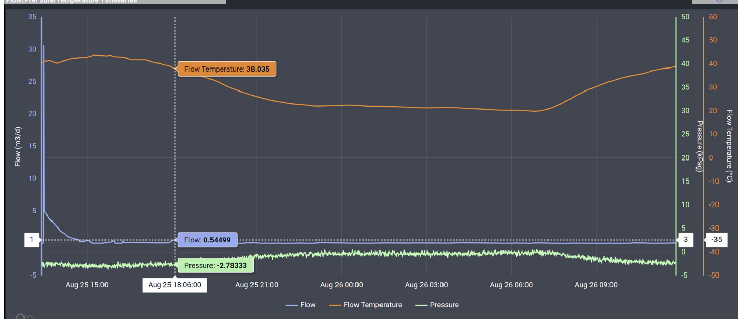
Image 4.1 – Twin Lakes SAU #095 (30-005-61107) Methane Flow/Pressure/Temperature Timeseries &amp; Peak Flow
