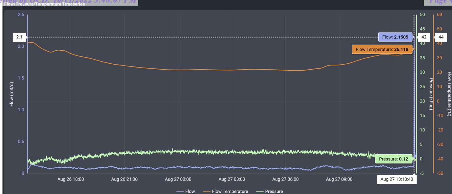
Image 4.1 – Twin Lakes SAU #099 (30-005-61261) Methane Flow/Pressure/Temperature Timeseries
