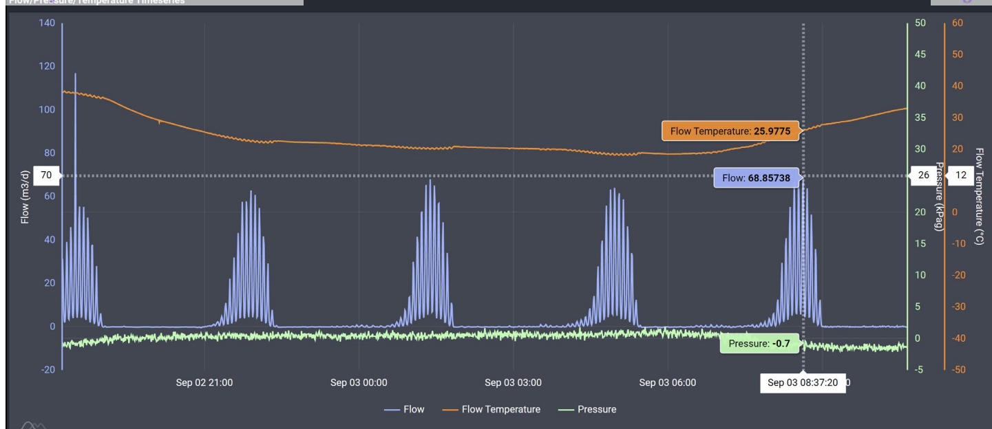
Image 4.1 – Double L Queen #02Z (30-005-60151) Methane Flow/Pressure/Temperature Timeseries &amp; Peak Flow
