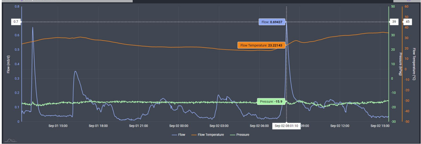
Image 4.1 – Double L Queen #01H (30-005-60127) Methane Flow/Pressure/Temperature Timeseries &amp; Peak Flow
