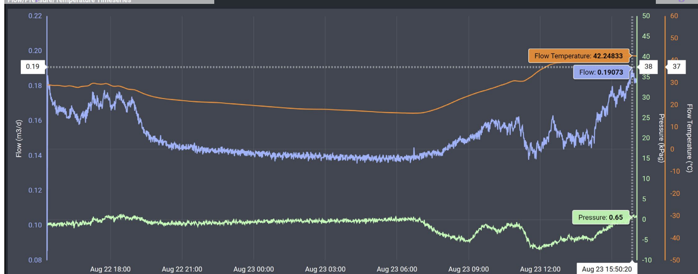
Image 4.1 – Twin Lakes SAU #061 (30-005-60920) Methane Flow/Pressure/Temperature Timeseries &amp; Peak Flow
