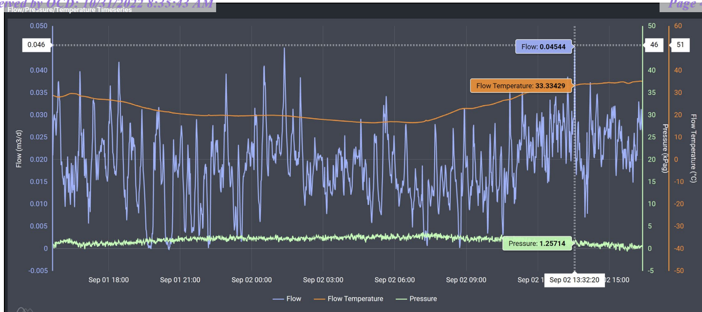
Image 4.1 – Double L Queen #04G (30-005-60080) Methane Flow/Pressure/Temperature Timeseries &amp; Peak Flow
