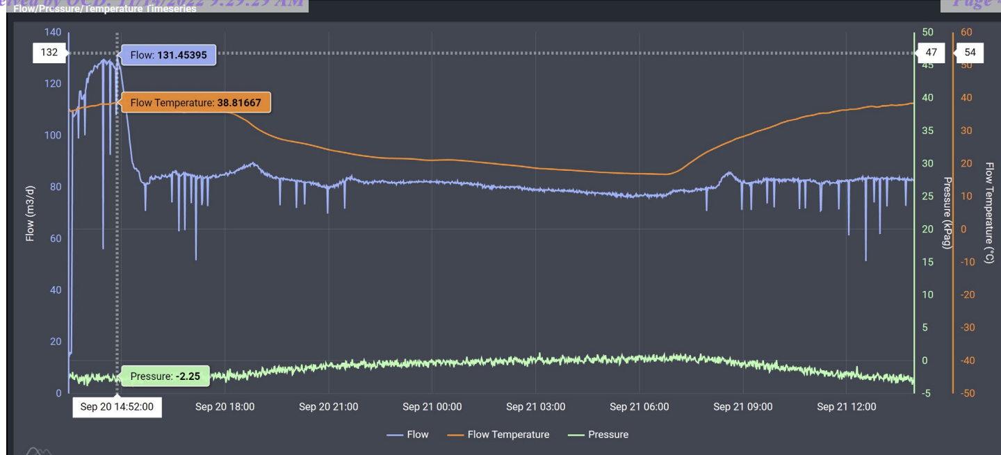
Image 4.1 – Cochise-King Gas Com #001 (30-025-30812) Methane Flow/Pressure/Temperature Timeseries &amp; Peak Flow
